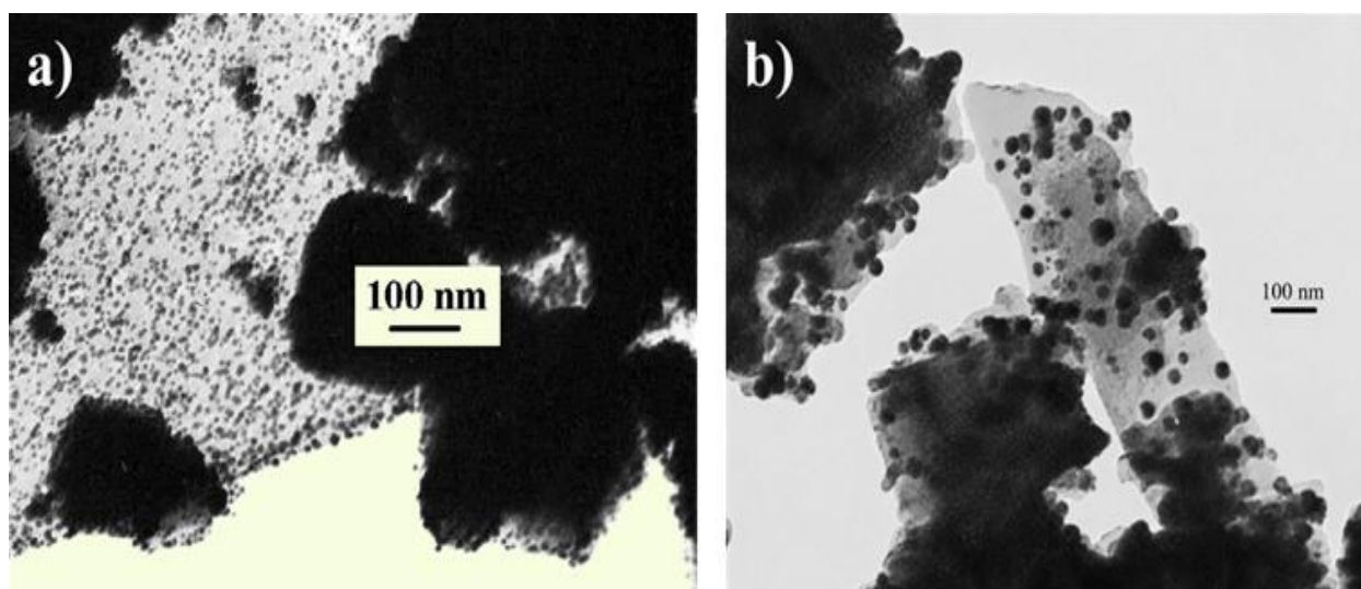
Figure 3 - Micrograph of 5% Pd/MgO catalysts: with (a) and without (b) P2M5VP [17]
