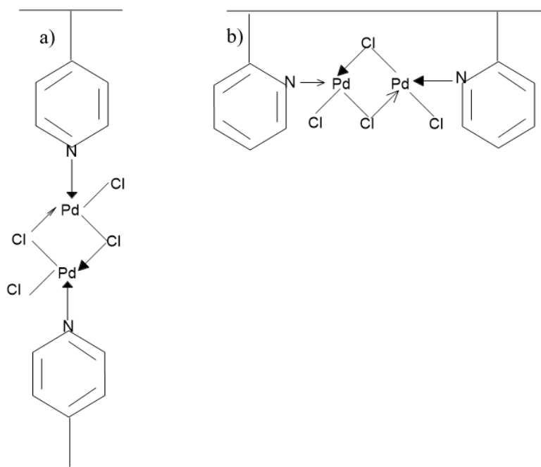
Figure 2 – Pd complexes with: a) P4VP, b) P2VP [13]
