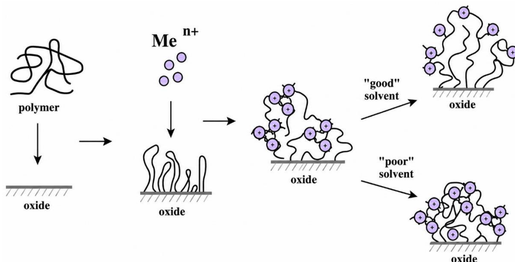
Figure 4 - Scheme for the preparation of PMC-on-oxide surface catalysts
