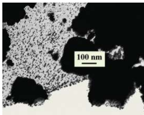
Figure 3 - Micrograph of 5% Pd–P2M5VP/MgO catalysts [10]
