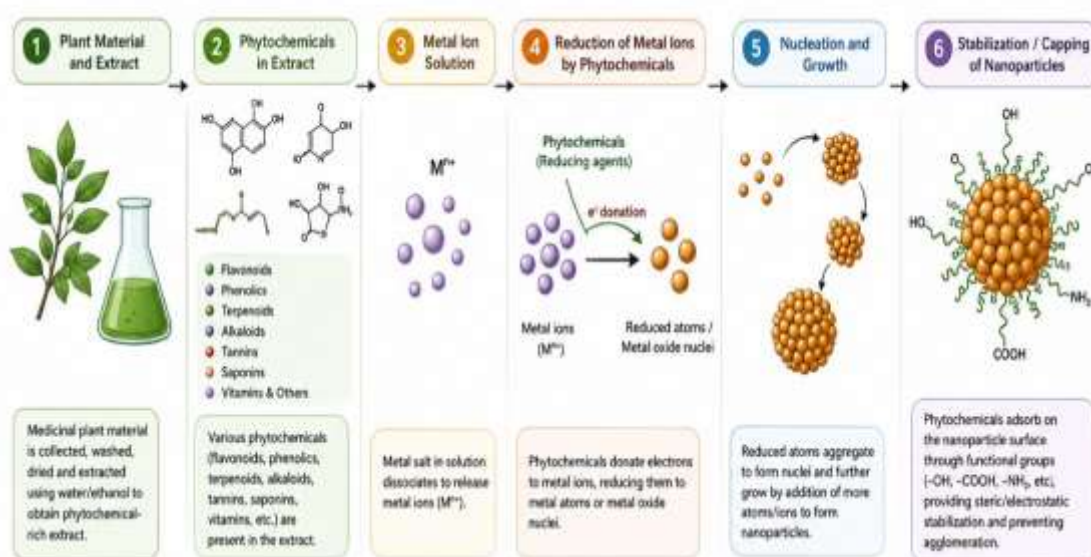
Figure 2 - Mechanism of Green Synthesis of Metal Oxide Nanoparticles Using Plant Extracts.
